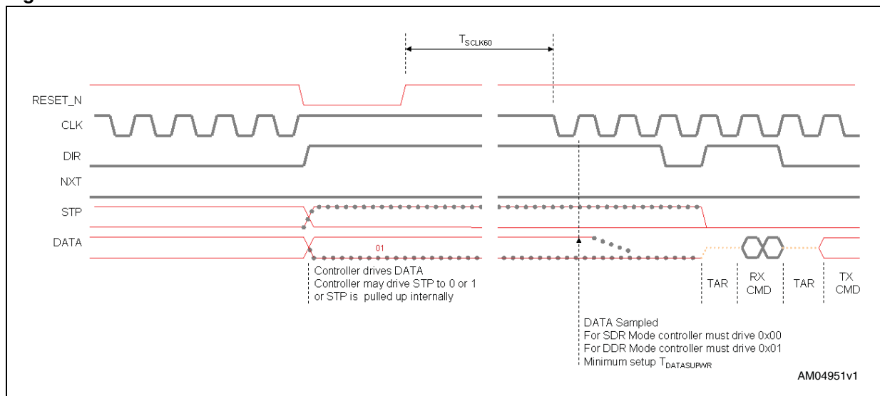
Figure 9. RESETn behavior
