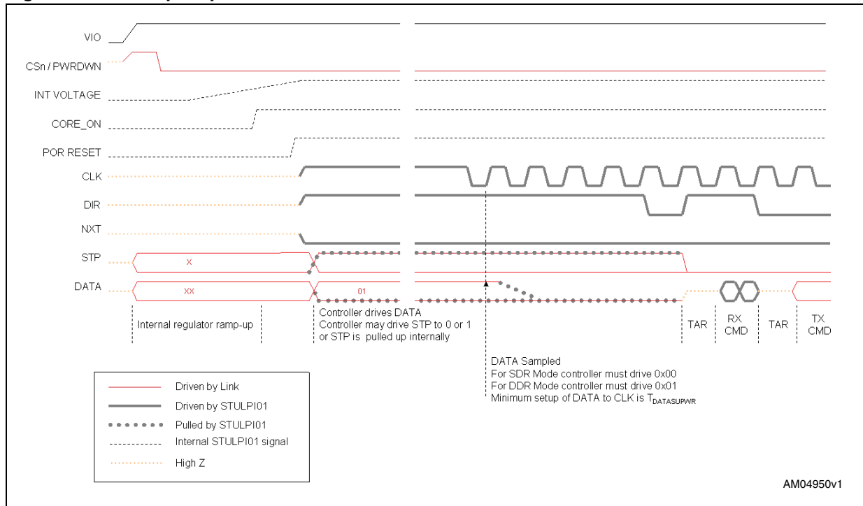
Figure 9. RESETn behavior
